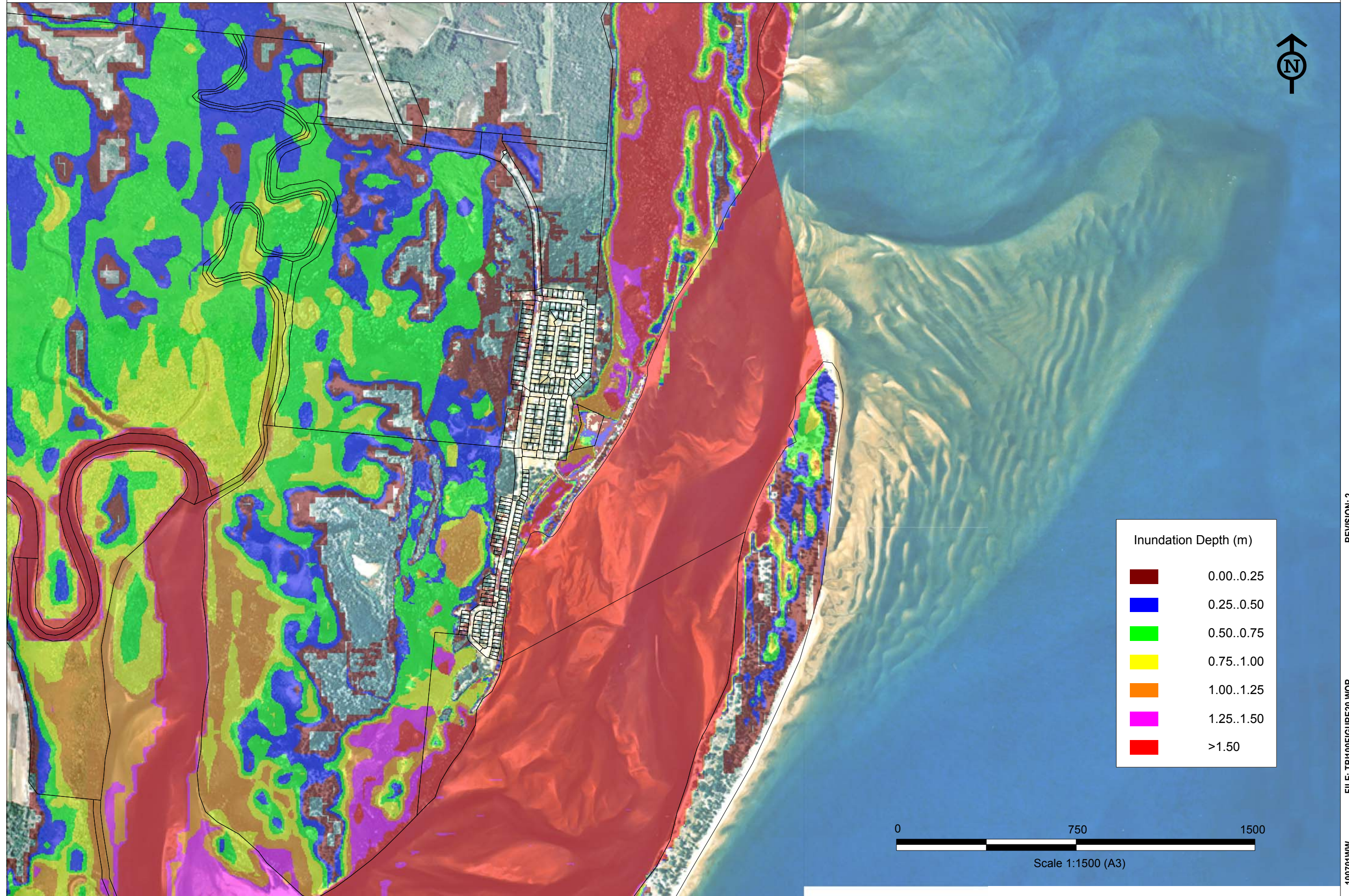
FIGURE 20: 100YR INUNDATION - TAYLORS BEACH
