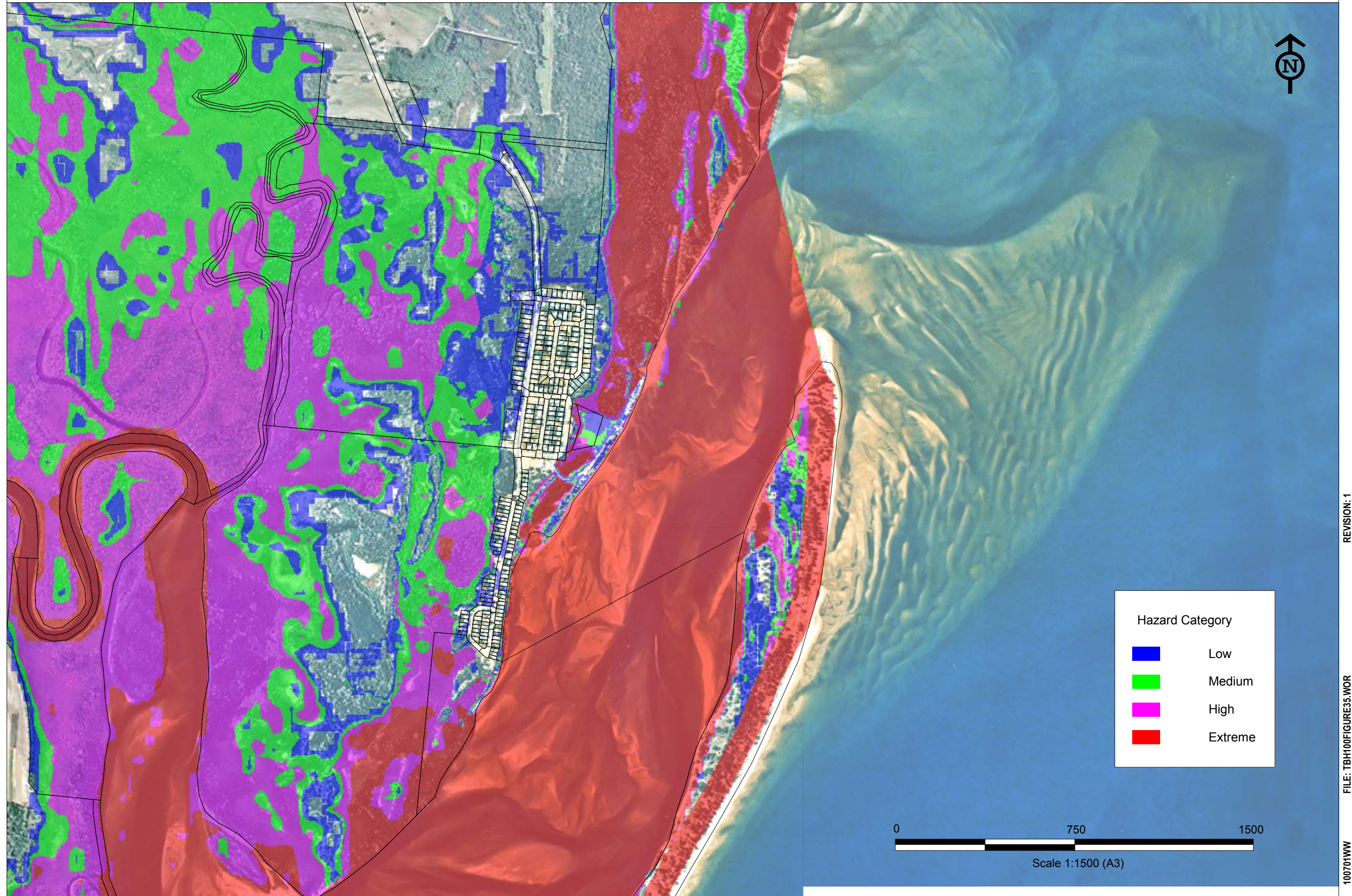
FIGURE 35: 100YR HAZARD - TAYLORS BEACH
